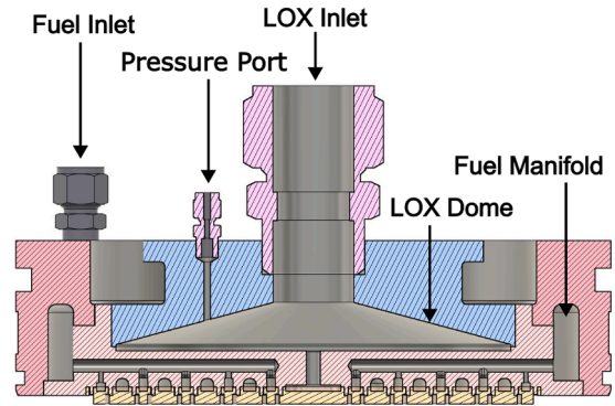
Fig. 12. Injector A final design cross-section.
